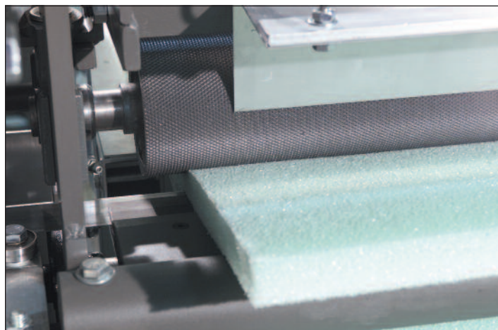
Adjustable pinch roller and heavy-duty blade guide
